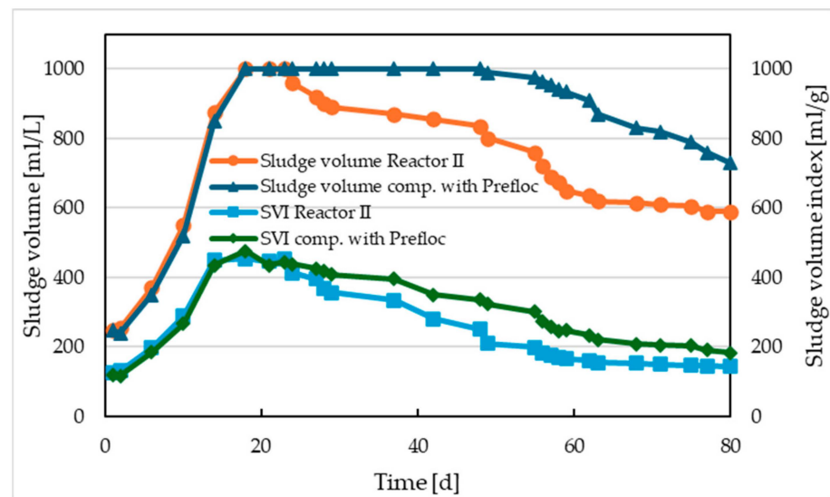
Figure 11. Sedimentation properties of activated sludge in Reactor II and in the comparative model with Prefloc dosing—sludge volume after 30 min of sedimentation and SVI.
