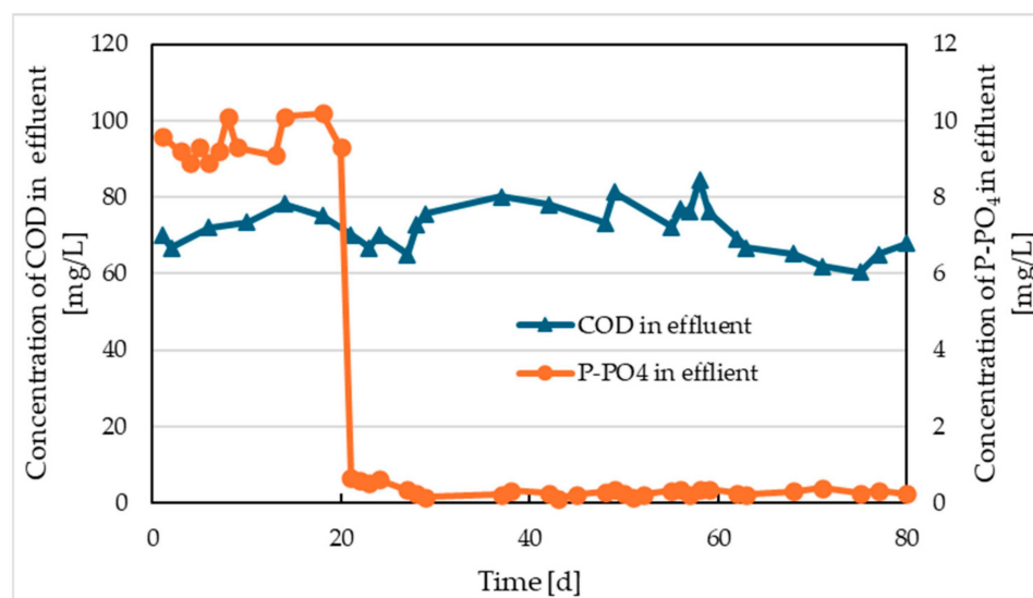
Figure 8. COD and \text{P-PO}_4 concentration in effluent from Reactor II.
