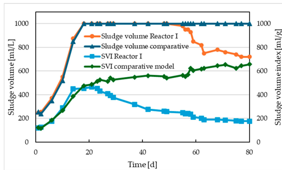
Figure 7. Sedimentation properties of activated sludge in Reactor I and in comparative model—sludge volume after 30 min of sedimentation and SVI.
