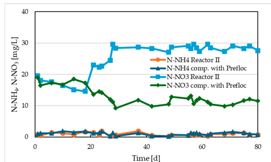
Figure 12. Course of \text{N-NH}_4 and \text{N-NO}_3 concentrations in effluent from Reactor II and from the comparative model with Prefloc dosing.
