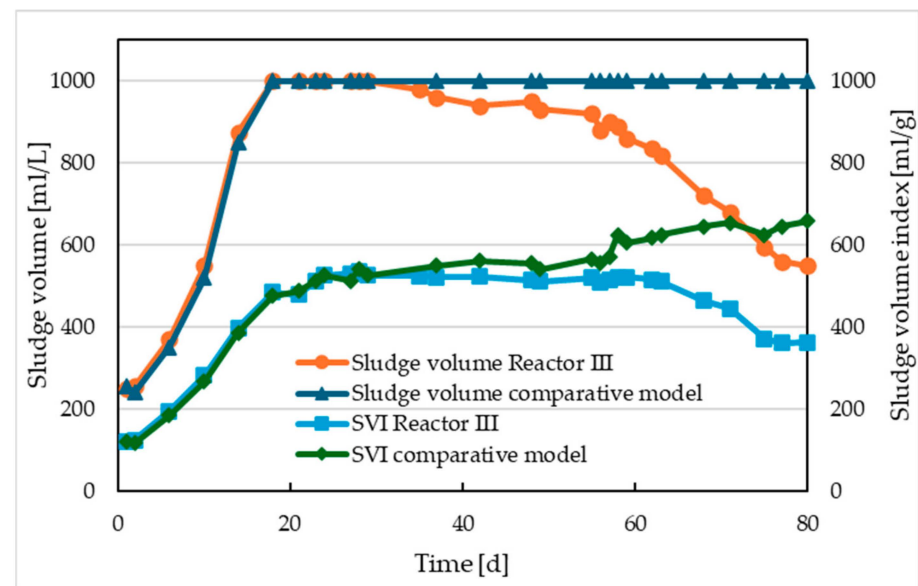
Figure 13. Sedimentation properties of activated sludge in Reactor III and in the comparative model—sludge volume after 30 min of sedimentation and SVI.
