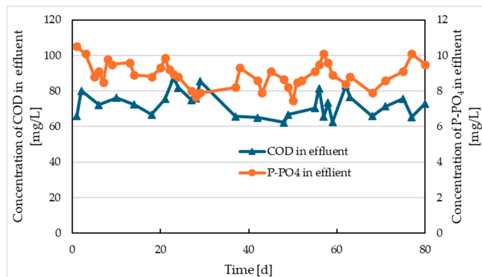
Figure 5. COD and P-PO 4 concentration in effluent from comparative model.
