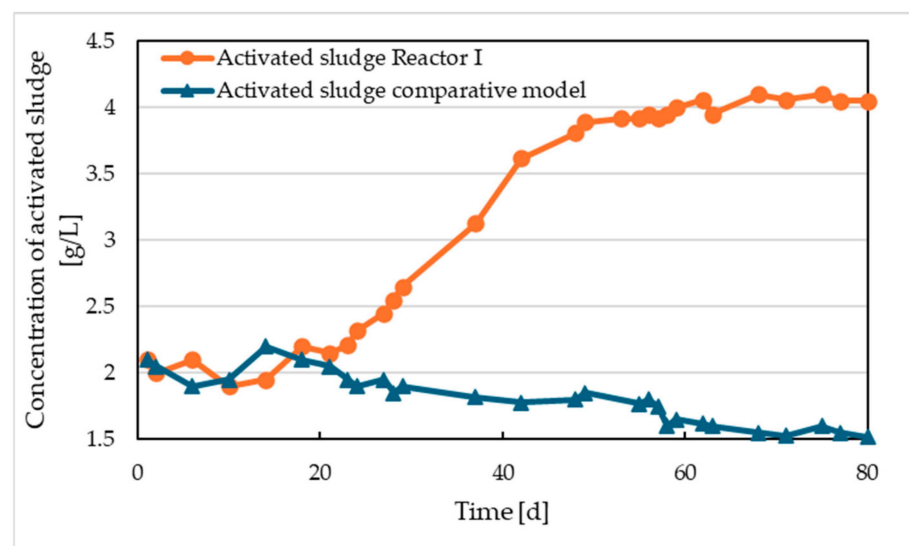
Figure 6. Activated sludge concentration in Reactor I and in the comparative model.
