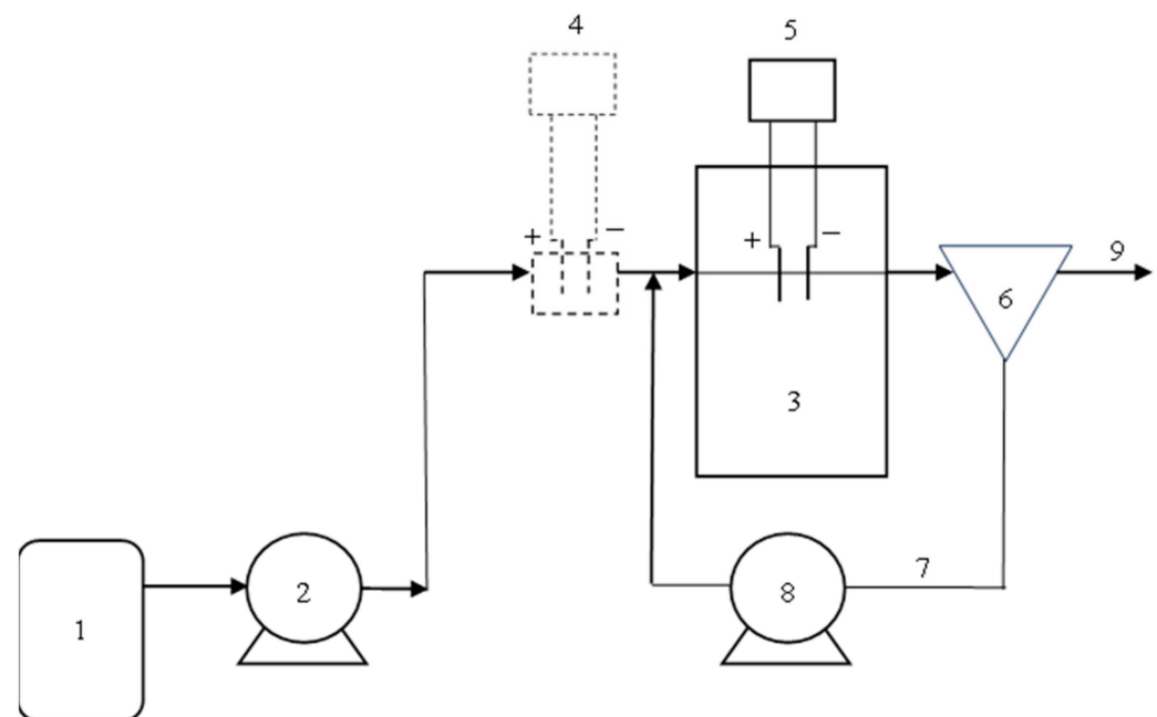
Figure 1. Scheme of laboratory model with electrolysis 1—stock solution (synthetic wastewater), 2—peristaltic pump, 3—activated sludge tank, 4—immersed electrodes with voltage source (alternative placement in separate tank), 5—immersed electrodes with voltage source (placement in activation), 6—sedimentation tank, 7—returned sludge, 8—peristaltic pump for sludge recirculation, 9—wastewater effluent.
