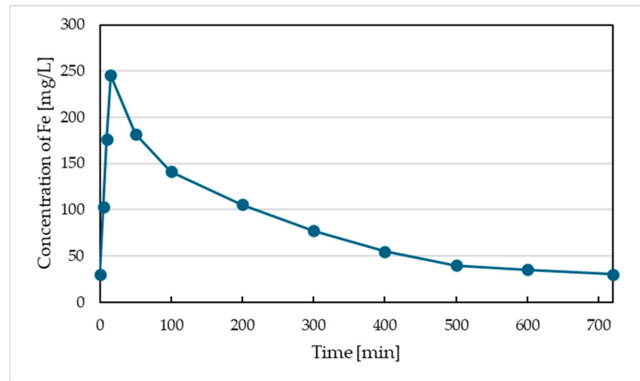
Figure 2. Concentration profile of iron in separate electrolysis.
