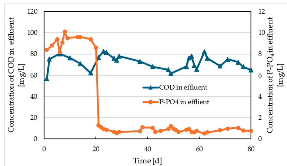
Figure 9. COD and P-PO 4 concentration in effluent from the comparative reactor with Prefloc dosing.
