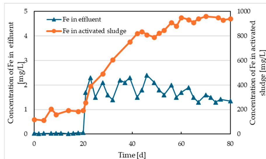
Figure 3. Course of Fe 2+ /Fe 3+ in the effluent and in the sludge from Reactor I.
