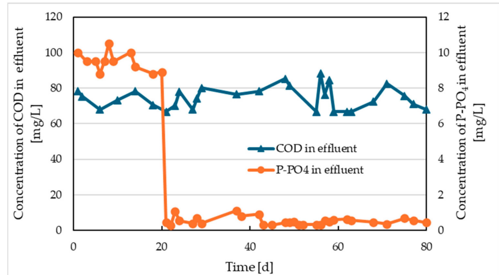
Figure 4. COD and P-PO 4 concentration in effluent from Reactor I.
