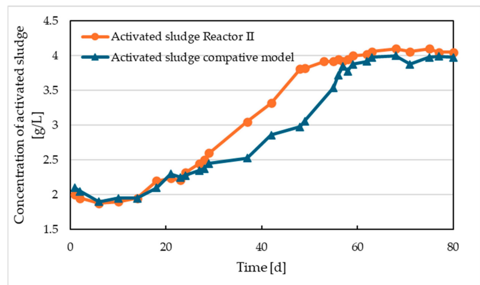
Figure 10. Concentration of activated sludge in Reactor II and in the comparative model with Prefloc dosing.
