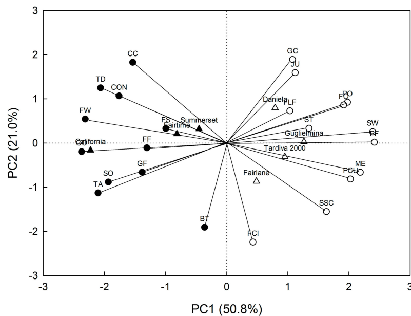
Figure 1. Two-dimensional positioning of cultivars (five peaches and two nectarines) and physical, chemical ( n = 30 ) and sensory ( n = 20 ) fruit quality attributes determined by Biplot technique (MDPREF). Trees (500/ha) were grown near Riesi ( 37^{\circ}16' N and 330 m a.s.l.), in central-southern Sicily. Open and closed symbols indicate the two groups obtained by k-means clustering of object and vector coordinates. FW, fresh weight; TD, transversal diameter; FF, flesh firmness; GC, ground color index; CC, percentage of cover color; SSC, soluble solid content; TA titratable acidity; ST, SSC/TA; PCU, peel color uniformity; CON, consistency; ES, easy stone; FCI, flesh color intensity; PO, peach odor; GO, grass odor; FO, flower odor; ME, mealiness; SW, sweetness; BT, bitterness; SO, sourness; JU, juiciness; PF, peach flavor; GF, grass flavor; FLF, flower flavor.
