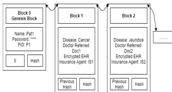
Figure 2. Patient Pat1 blockchain.
