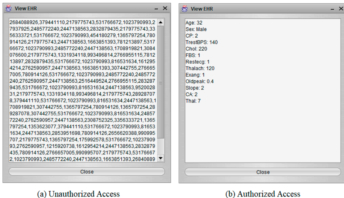
Figure 5. EHRs as a result of unauthorized access vs. authorized access.
